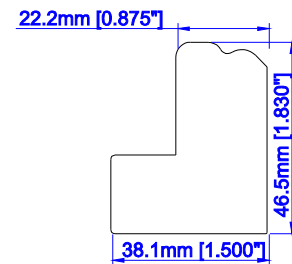
3" Crown Z Sill Plate
