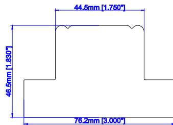
1 3/4" T Post W/ 3/4" Light Block (L/Z/HS)
