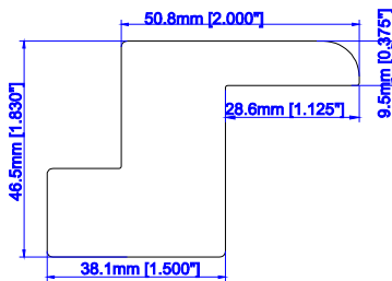
2" Bullnose Z Frame
