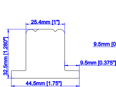
1" T Post W/ 1/4" Thick 3/8" Wide Light Block (Deco)
