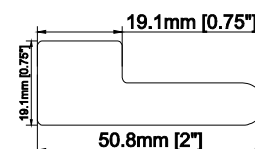
2" Sill Plate with 3/8" Light Block (L/Z)
