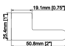
2" Sill Plate with 5/8" Light Block (L/Z)
