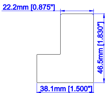
1 1/2" Bullnose Z 1 1/4" Beaded Z Sill Plate
