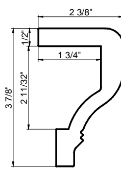
Curved Designer Sill Cap (D/HS)
