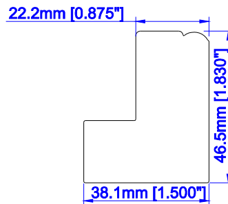
2" Bel Air Z Sill Plate
