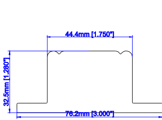
1 3/4" T Post W/ 1/4" Light Block (Deco)
